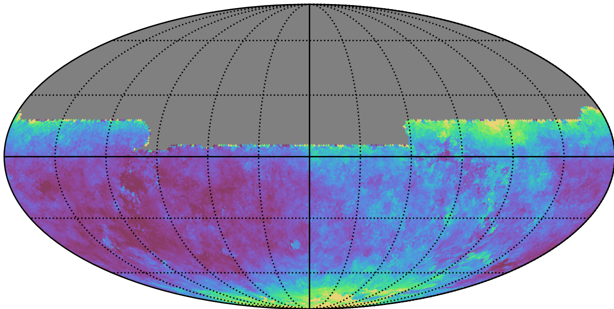
baseline_v3.3_10yrs All sky y band: Median seeingEff
