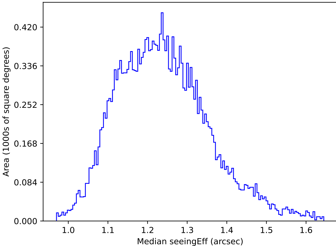
baseline_v3.3_10yrs All sky u band: Median seeingEff
