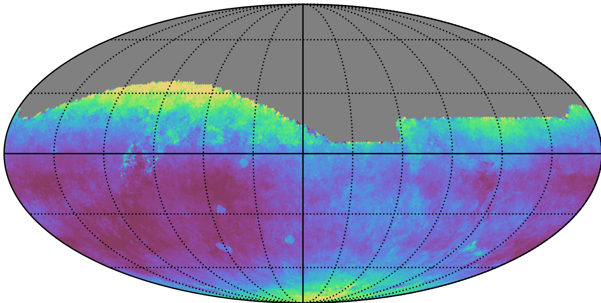
baseline_v3.3_10yrs All sky r band: Median seeingEff
