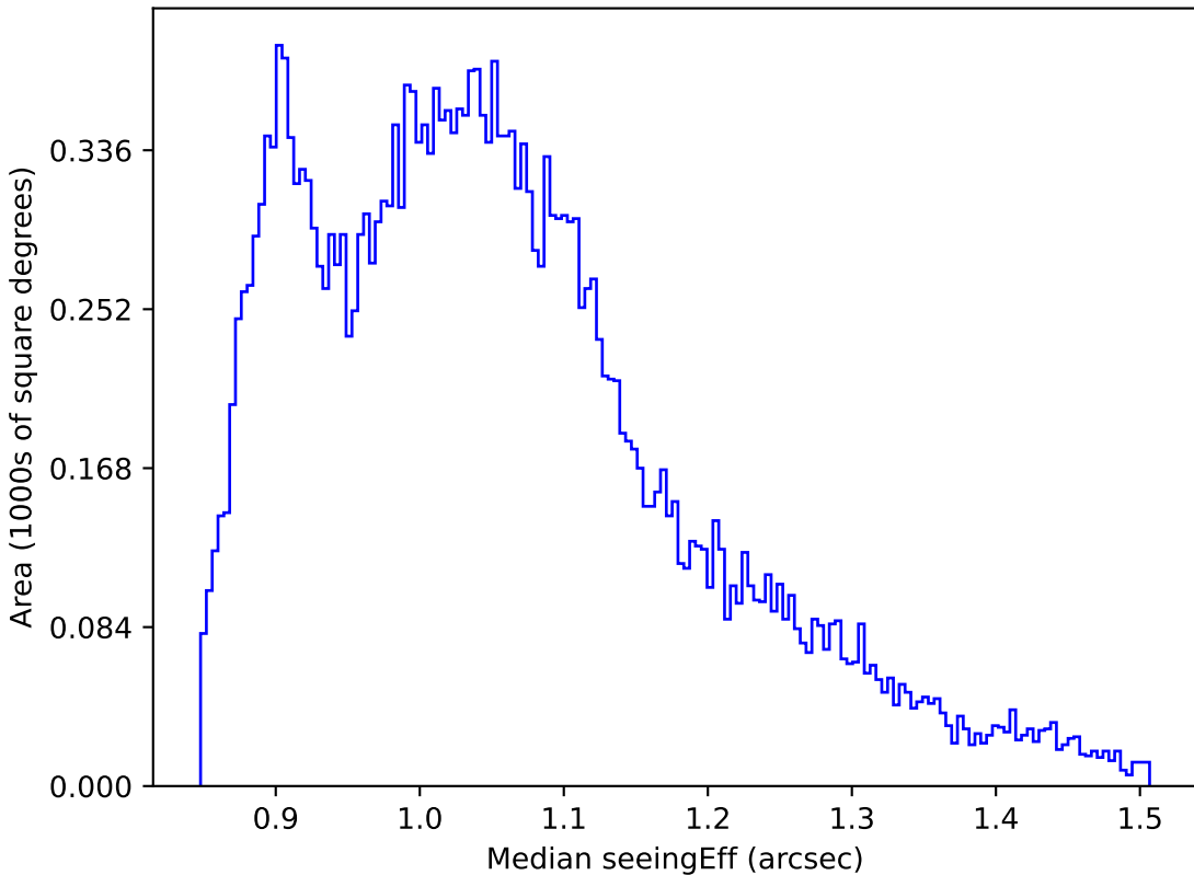
baseline_v3.3_10yrs All sky r band: Median seeingEff
