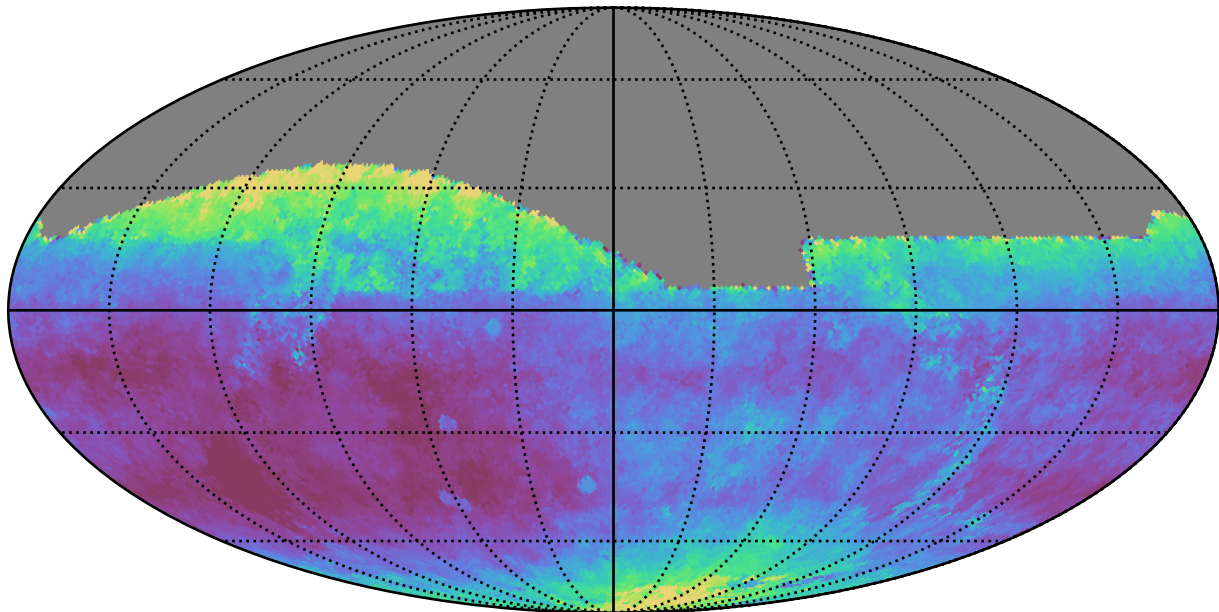
baseline_v3.3_10yrs All sky i band: Median seeingEff
