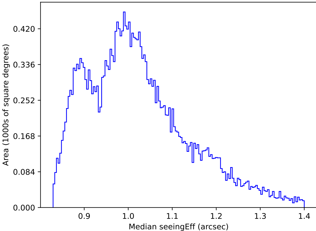
baseline_v3.3_10yrs All sky i band: Median seeingEff
