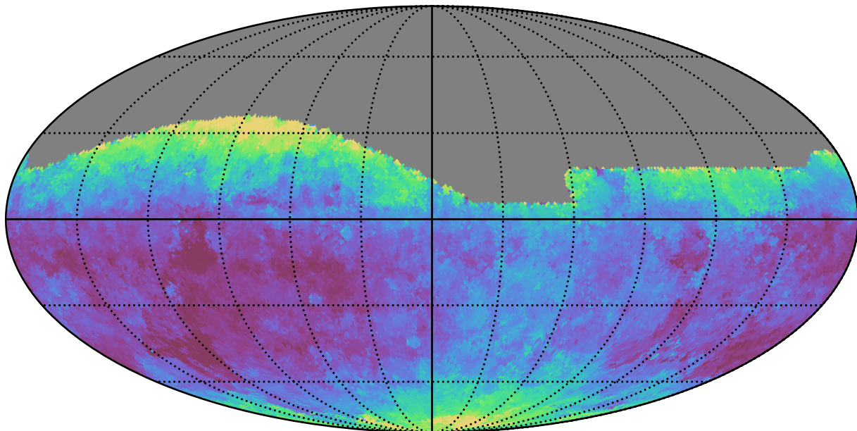
baseline_v3.3_10yrs All sky g band: Median seeingEff
