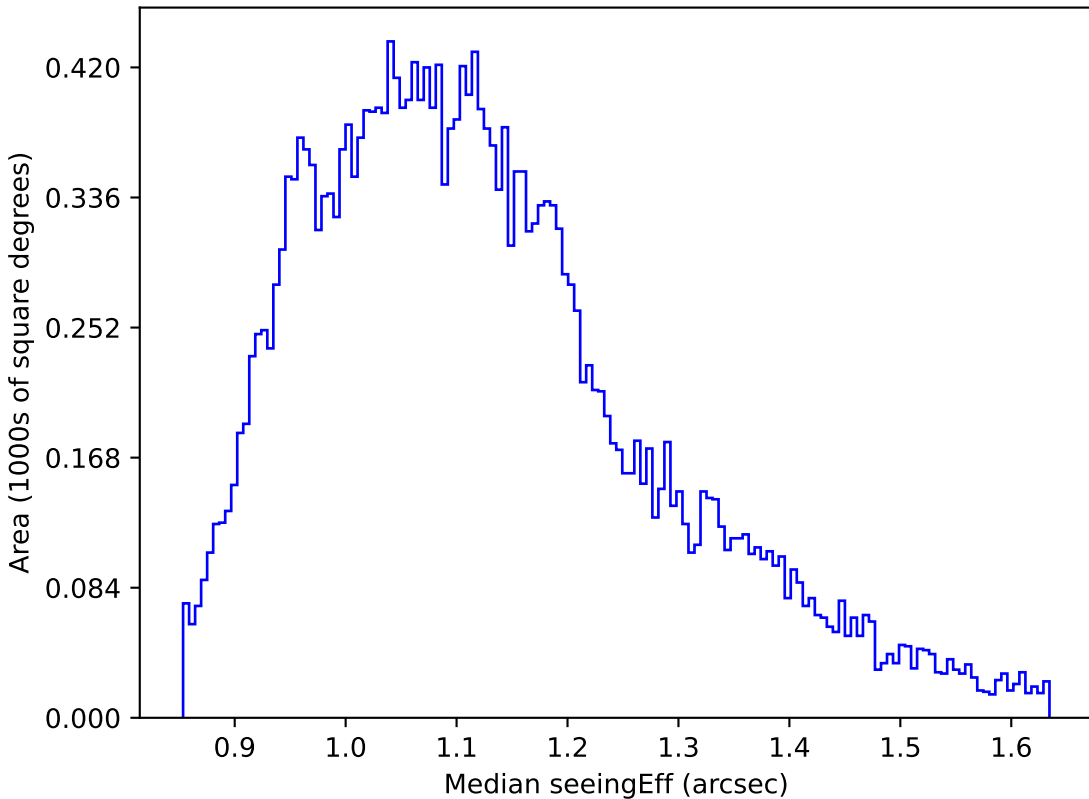
baseline_v3.3_10yrs All sky g band: Median seeingEff
