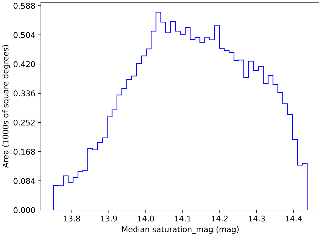
baseline_v3.3_10yrs WFD z band: Median saturation_mag
