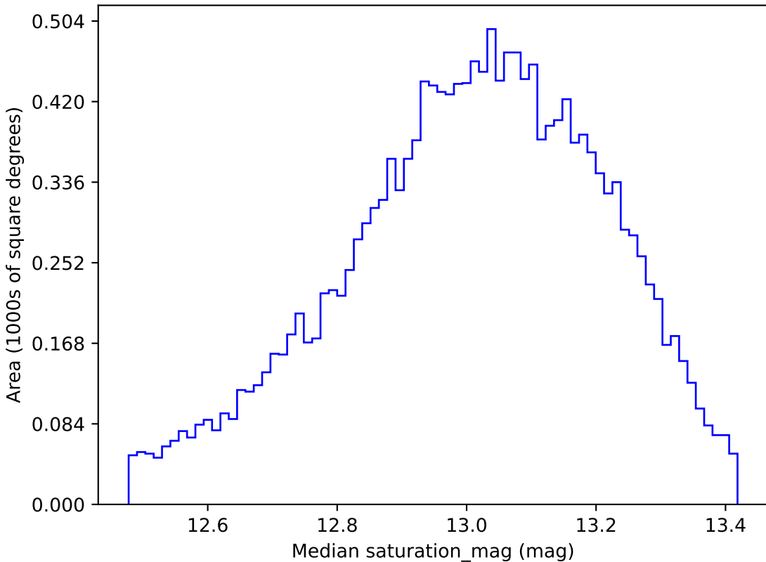
baseline_v3.3_10yrs WFD u band: Median saturation_mag
