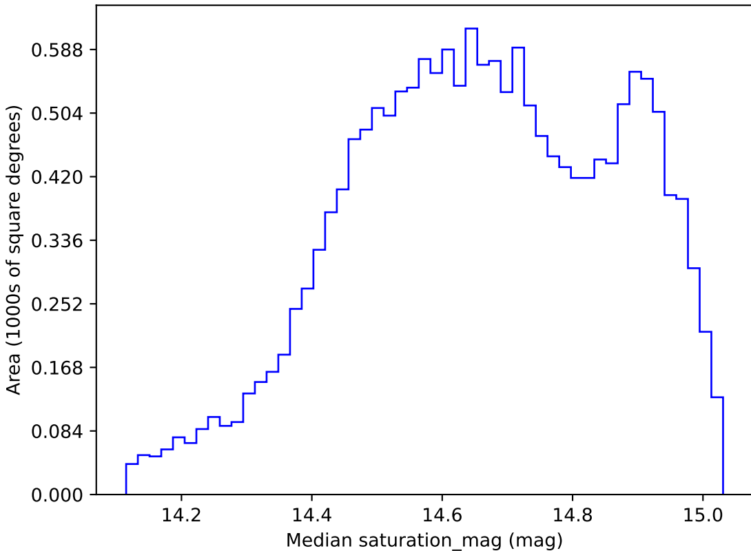
baseline_v3.3_10yrs WFD r band: Median saturation_mag
