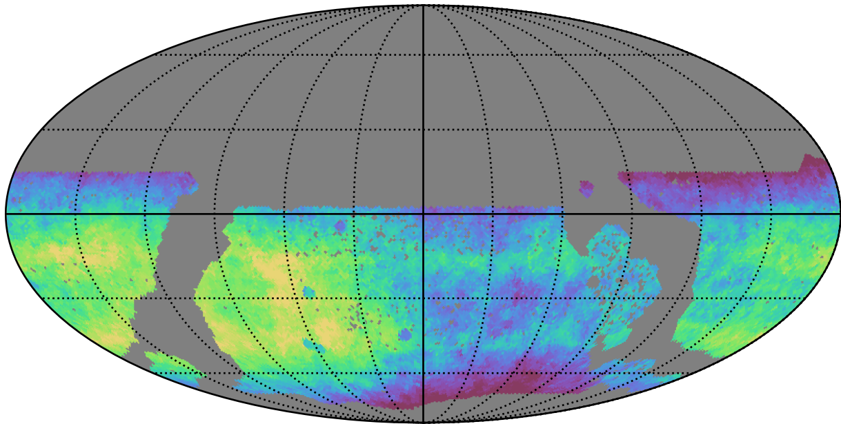
baseline_v3.3_10yrs WFD i band: Median saturation_mag
