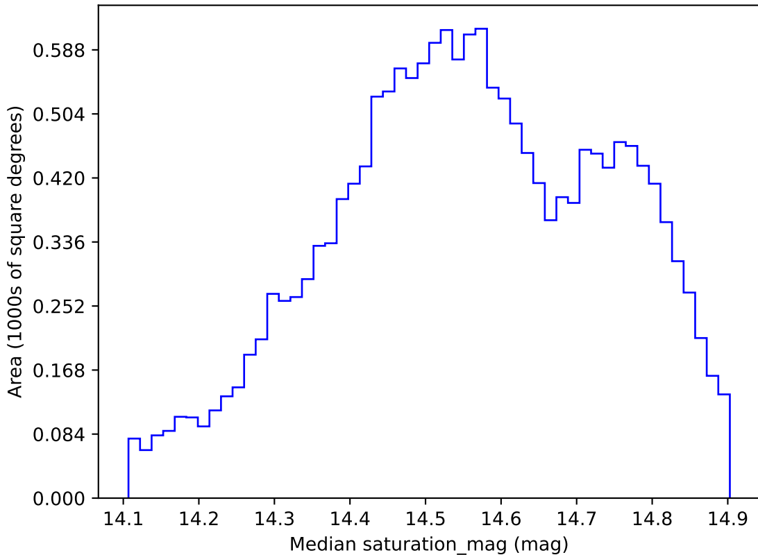
baseline_v3.3_10yrs WFD i band: Median saturation_mag
