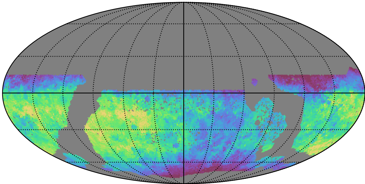
baseline_v3.3_10yrs WFD g band: Median saturation_mag
