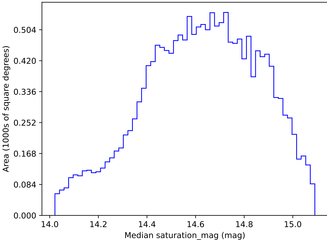
baseline_v3.3_10yrs WFD g band: Median saturation_mag
