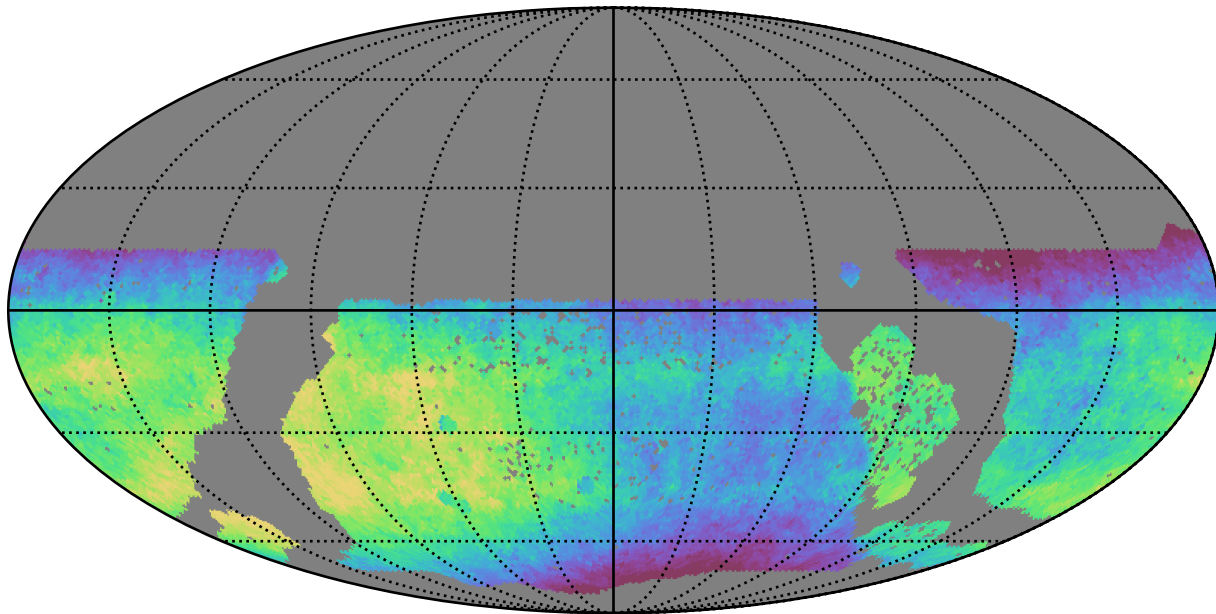
baseline_v3.3_10yrs WFD all bands: Median saturation_mag
