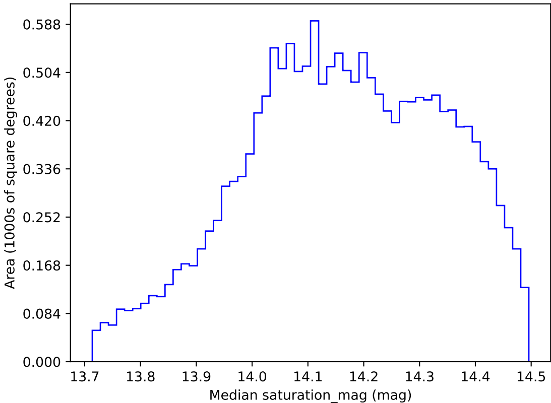
baseline_v3.3_10yrs WFD all bands: Median saturation_mag
