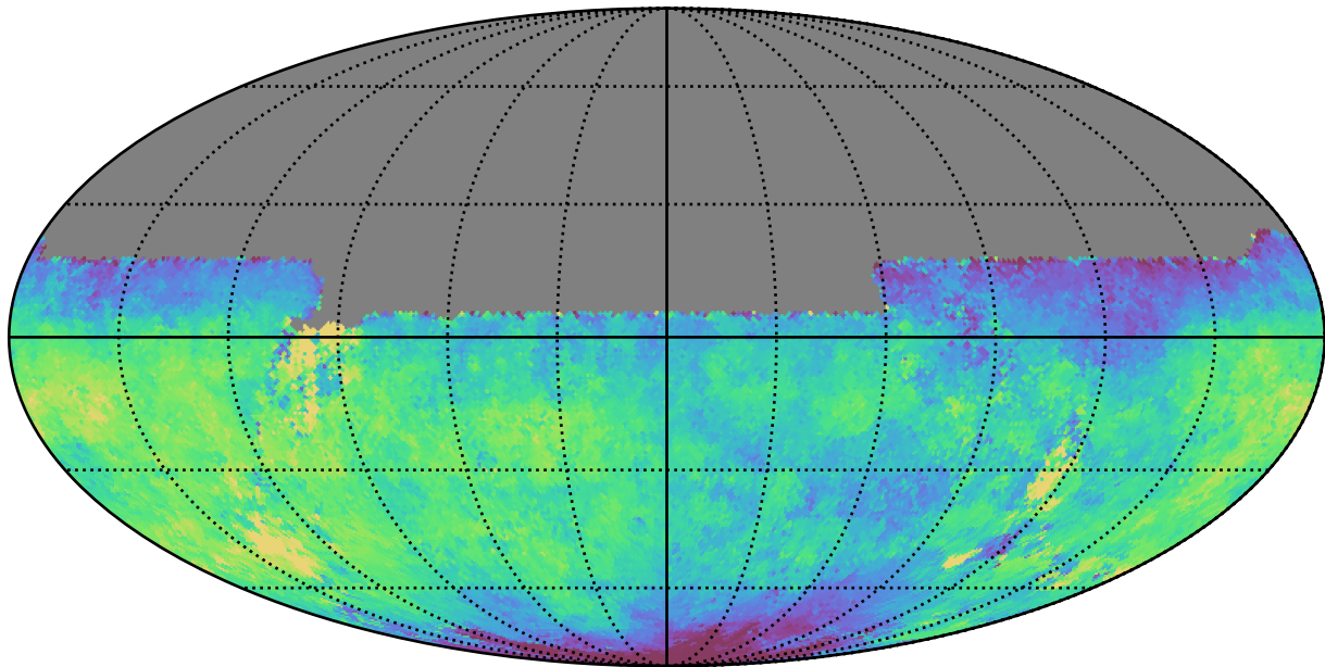
baseline_v3.3_10yrs All sky u band: Median saturation_mag
