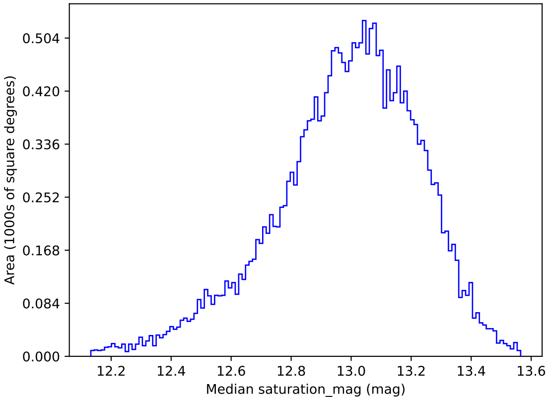
baseline_v3.3_10yrs All sky u band: Median saturation_mag
