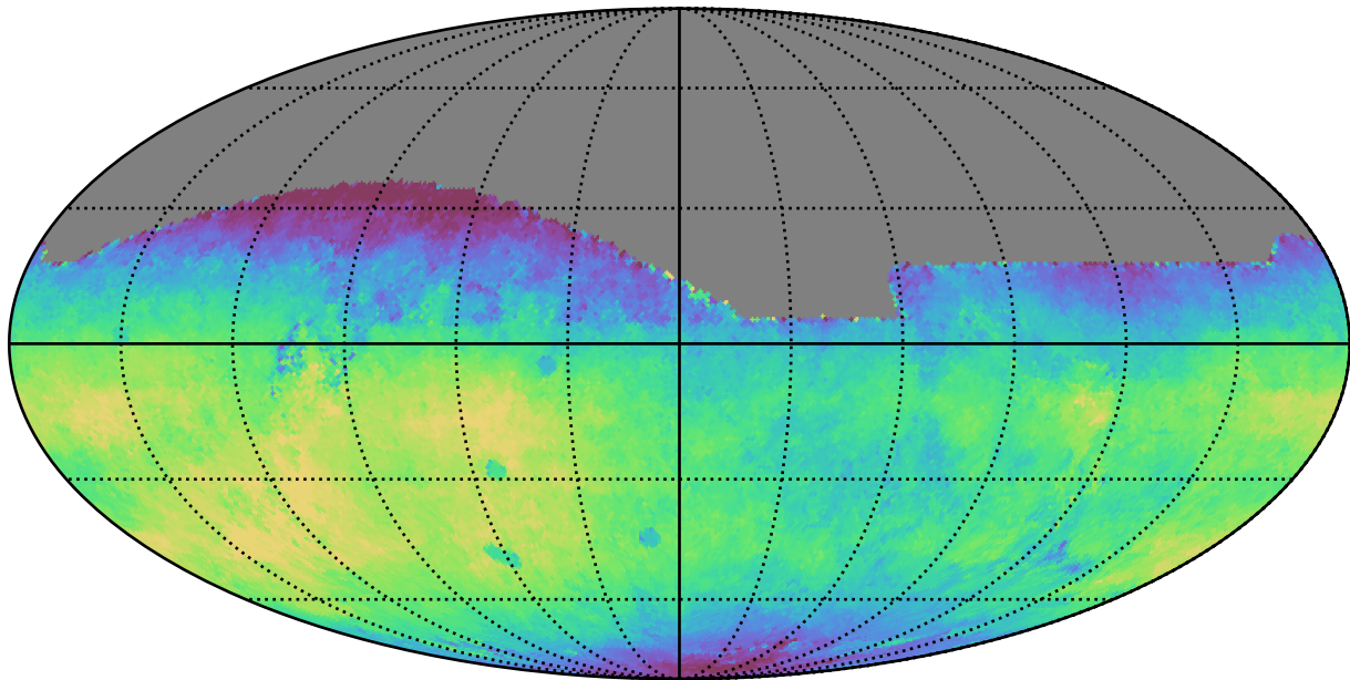
baseline_v3.3_10yrs All sky r band: Median saturation_mag
