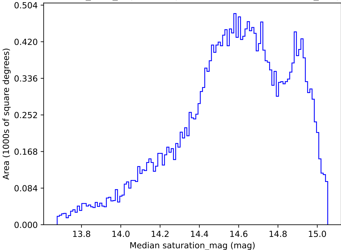
baseline_v3.3_10yrs All sky r band: Median saturation_mag
