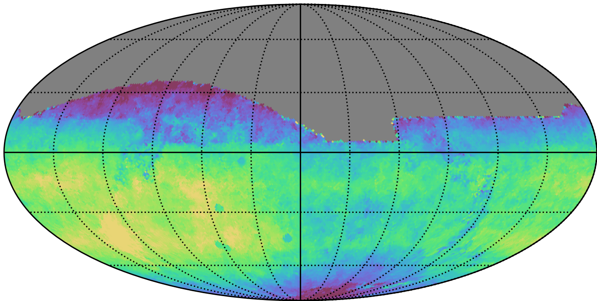
baseline_v3.3_10yrs All sky i band: Median saturation_mag
