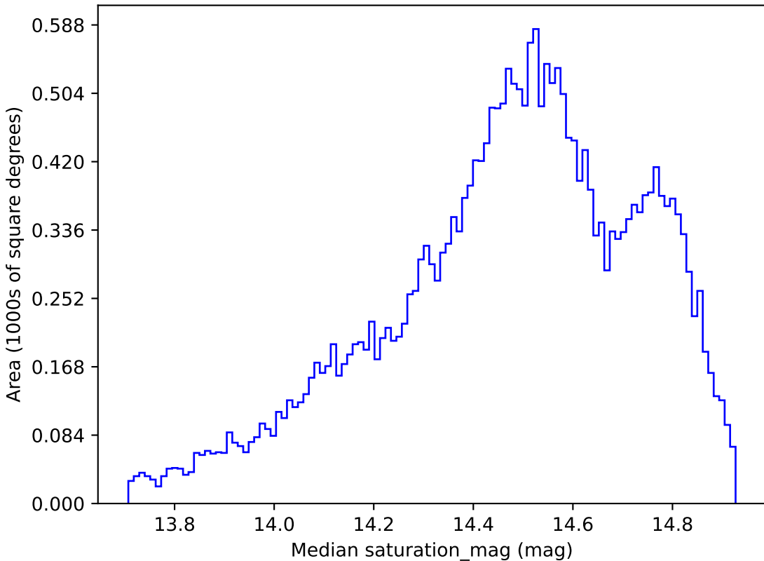
baseline_v3.3_10yrs All sky i band: Median saturation_mag
