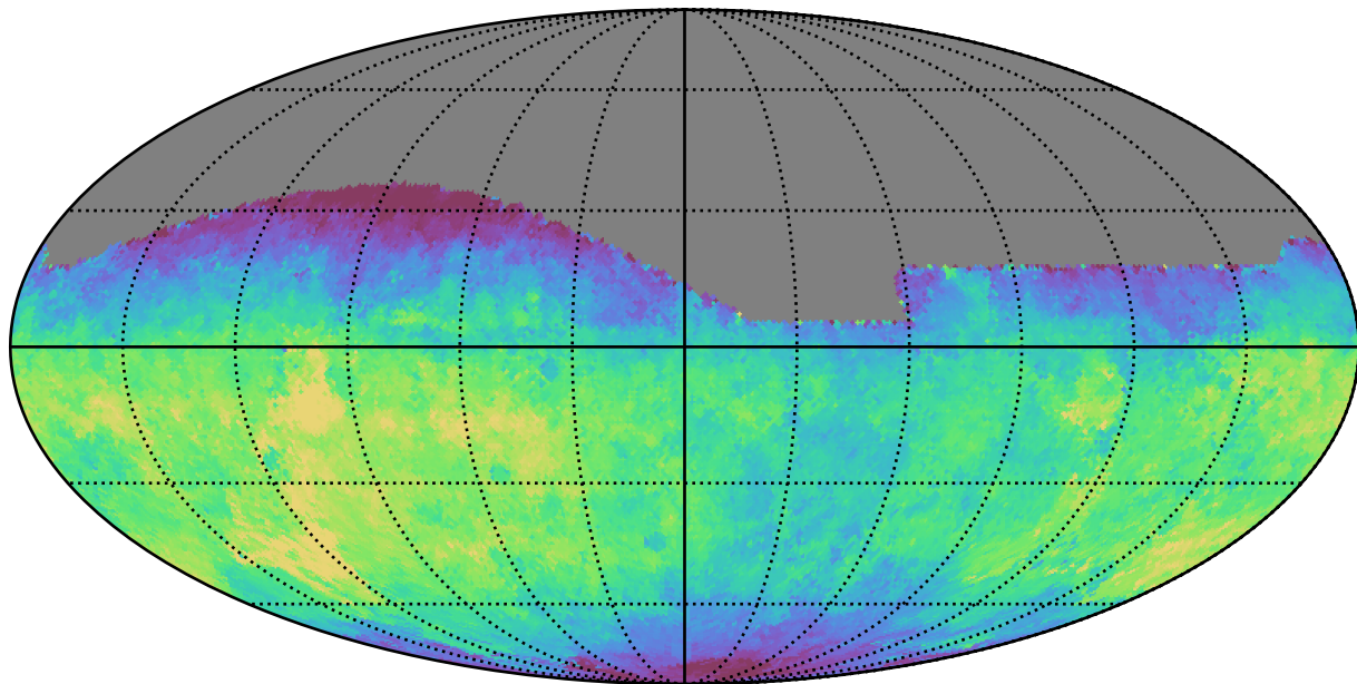
baseline_v3.3_10yrs All sky g band: Median saturation_mag
