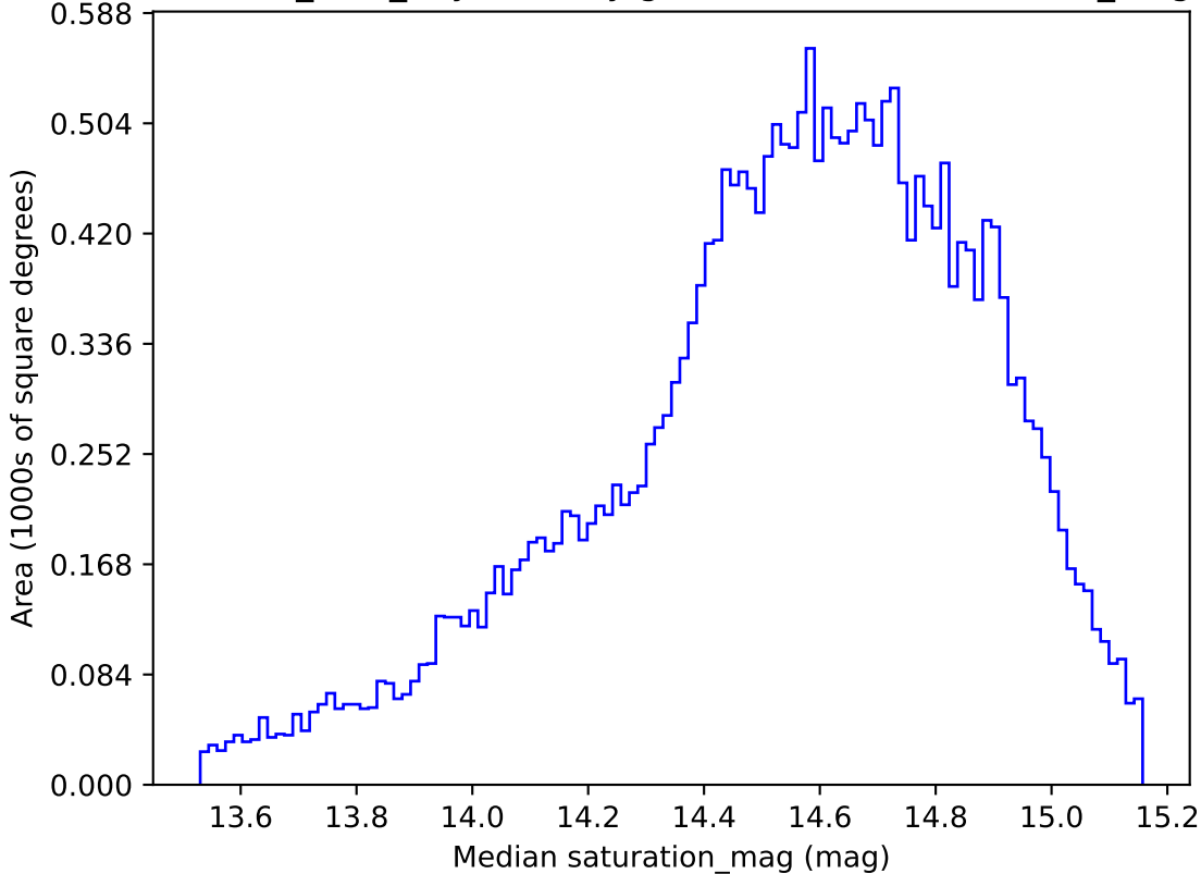
baseline_v3.3_10yrs All sky g band: Median saturation_mag
