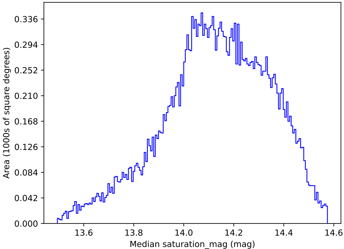
baseline_v3.3_10yrs All sky all bands: Median saturation_mag
