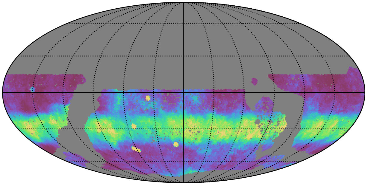
baseline_v3.3_10yrs WFD z band: Median normairmass
