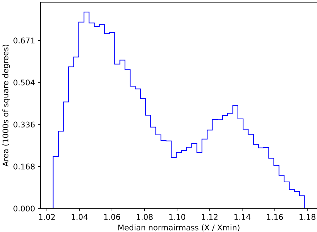
baseline_v3.3_10yrs WFD y band: Median normairmass
