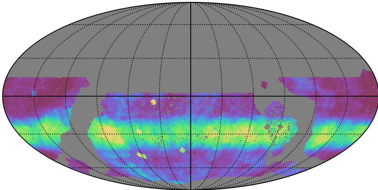
baseline_v3.3_10yrs WFD r band: Median normairmass
