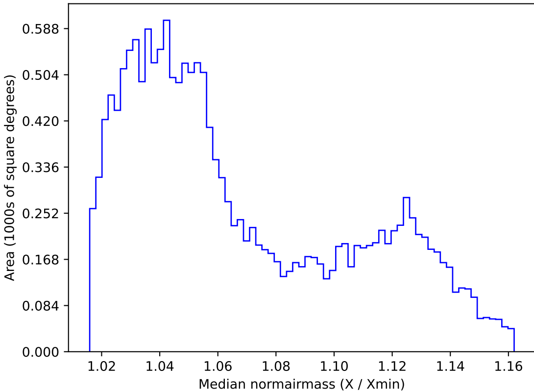
baseline_v3.3_10yrs WFD r band: Median normairmass
