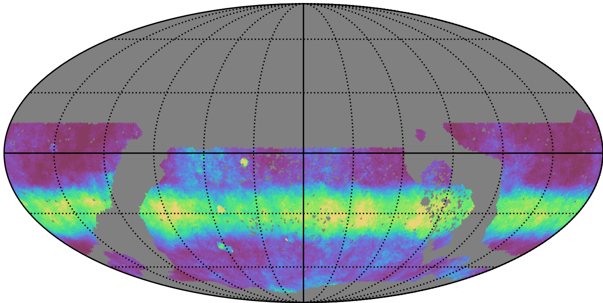
baseline_v3.3_10yrs WFD i band: Median normairmass
