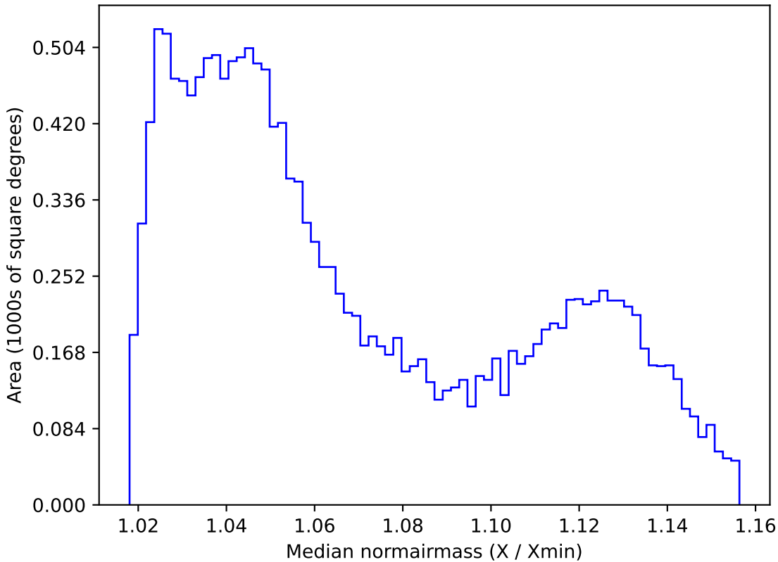
baseline_v3.3_10yrs WFD i band: Median normairmass
