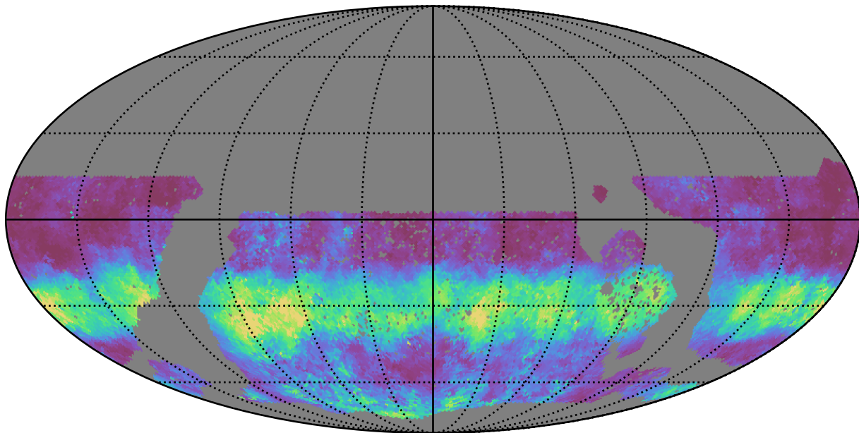
baseline_v3.3_10yrs WFD g band: Median normairmass
