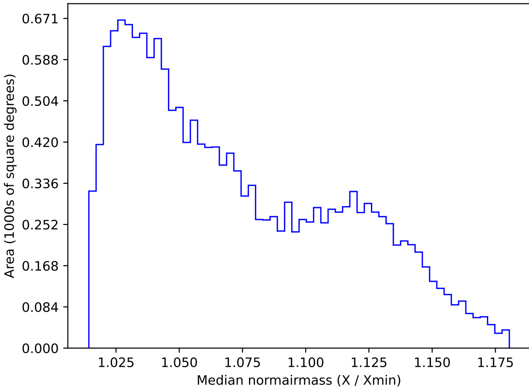
baseline_v3.3_10yrs WFD g band: Median normairmass
