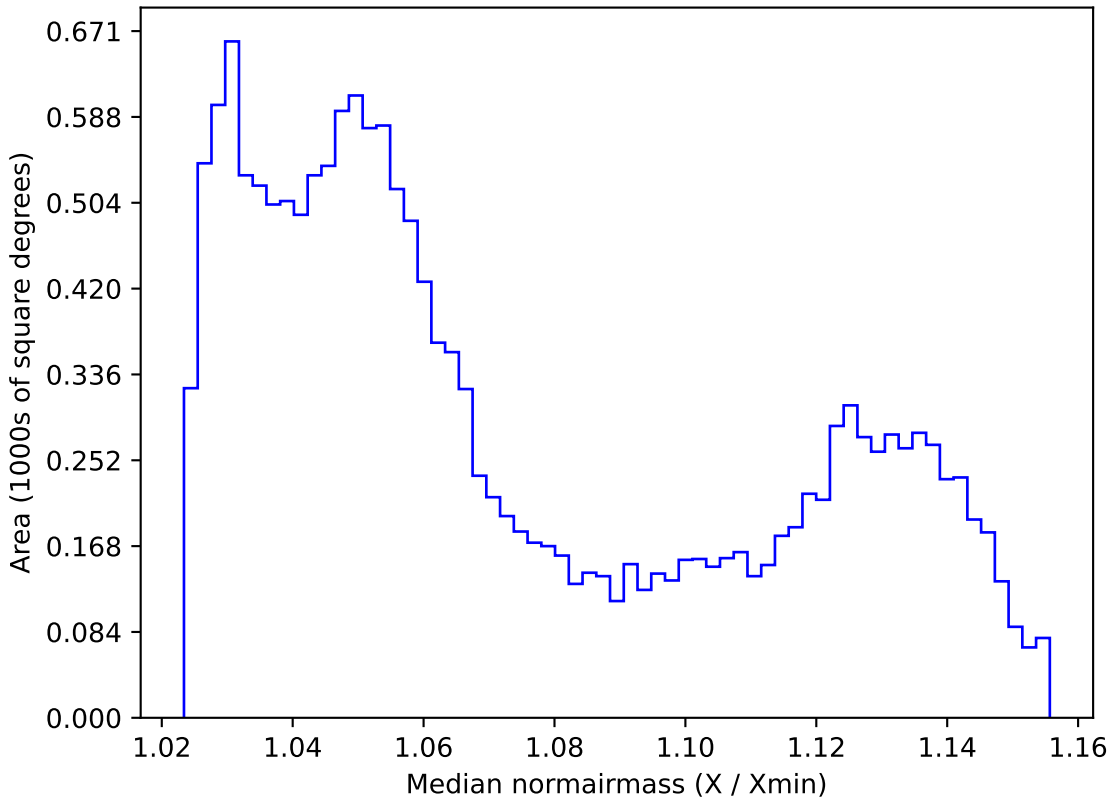
baseline_v3.3_10yrs WFD all bands: Median normairmass
