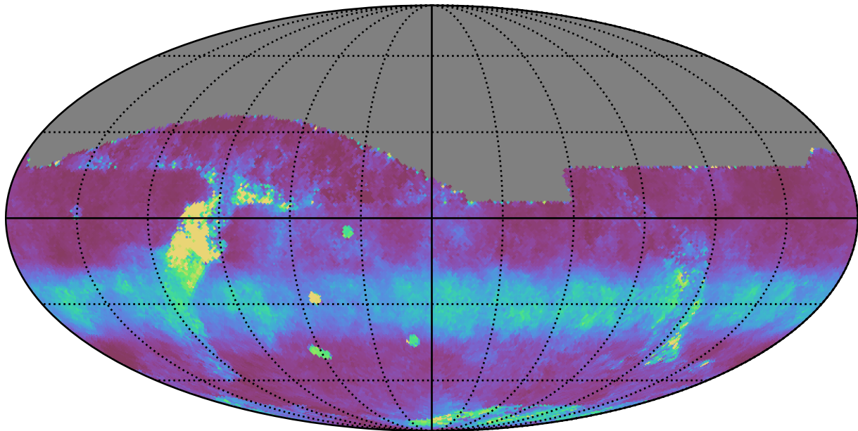
baseline_v3.3_10yrs All sky z band: Median normairmass
