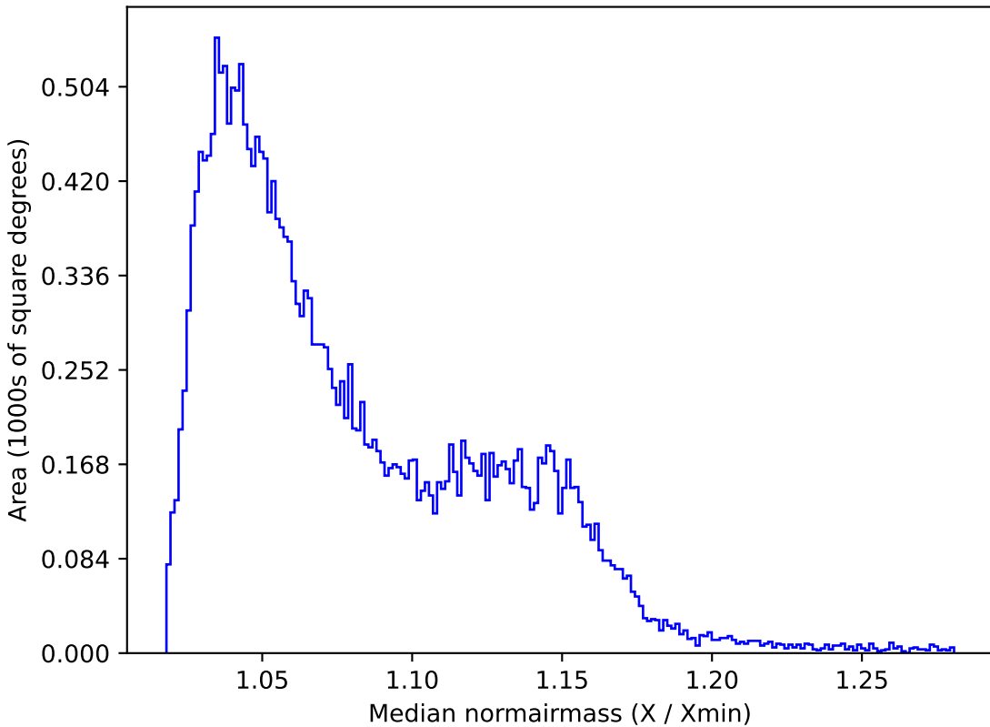
baseline_v3.3_10yrs All sky z band: Median normairmass
