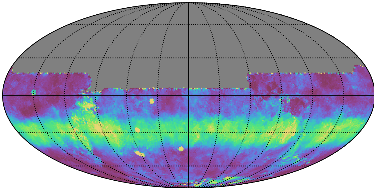
baseline_v3.3_10yrs All sky y band: Median normairmass
