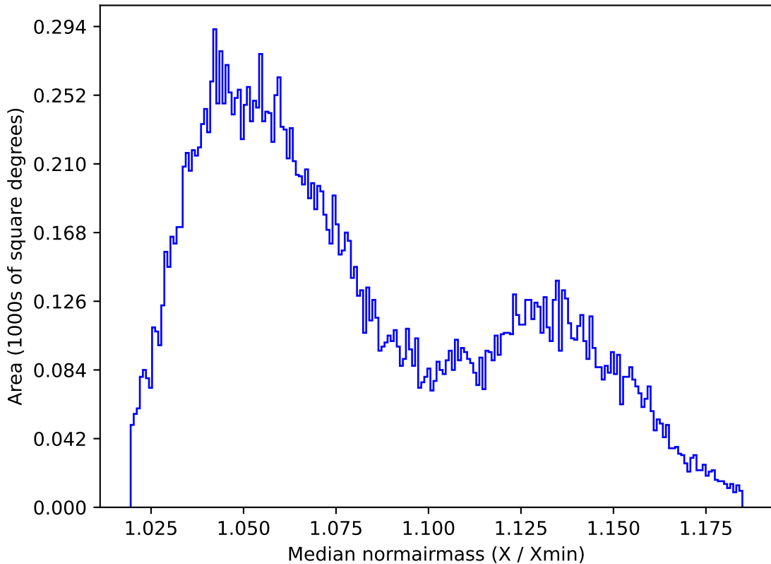
baseline_v3.3_10yrs All sky y band: Median normairmass
