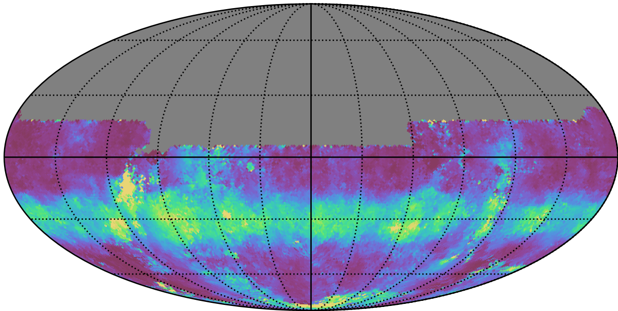
baseline_v3.3_10yrs All sky u band: Median normairmass
