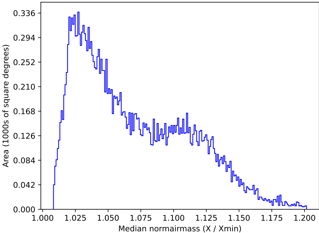
baseline_v3.3_10yrs All sky u band: Median normairmass
