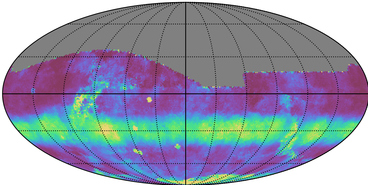
baseline_v3.3_10yrs All sky r band: Median normairmass
