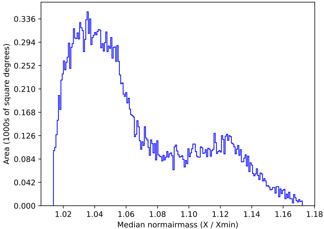
baseline_v3.3_10yrs All sky r band: Median normairmass
