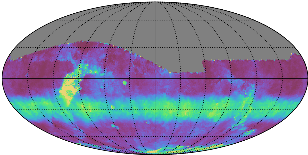
baseline_v3.3_10yrs All sky i band: Median normairmass
