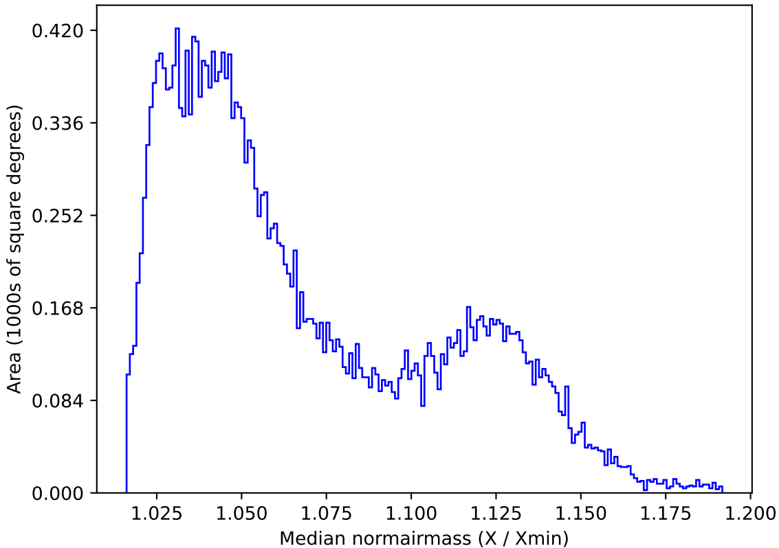
baseline_v3.3_10yrs All sky i band: Median normairmass
