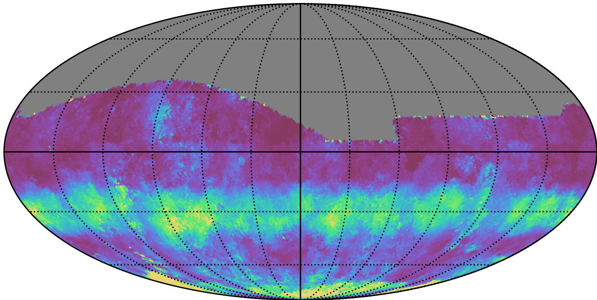
baseline_v3.3_10yrs All sky g band: Median normairmass
