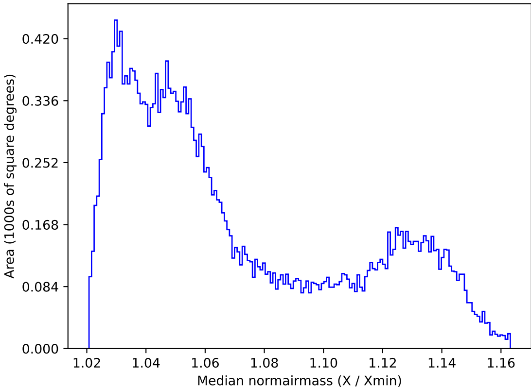
baseline_v3.3_10yrs All sky all bands: Median normairmass
