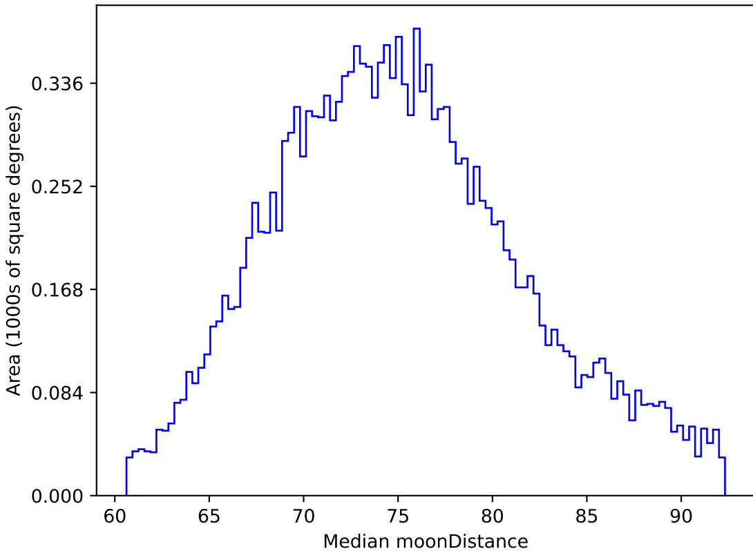
baseline_v3.3_10yrs WFD z band: Median moonDistance
