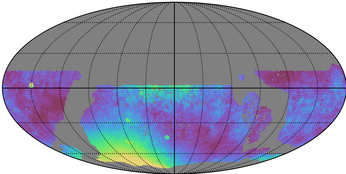
baseline_v3.3_10yrs WFD y band: Median moonDistance
