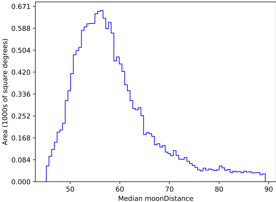
baseline_v3.3_10yrs WFD y band: Median moonDistance
